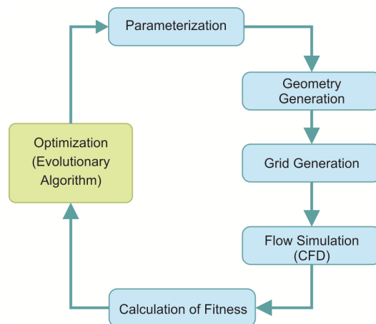
Fig. 2: Numerical process chain for the optimisation of the flow and temperature profiles at long range.
