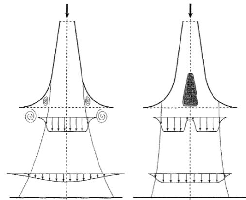
Fig.1: Illustration of the effect of a central body in the nozzle outlet (right) compared with a conventional nozzle.
