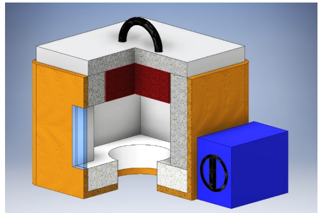
Figure: CAD model of the first prototype design of the hand-held device for on-site testing of intumescent coatings [Picture: KIT].
