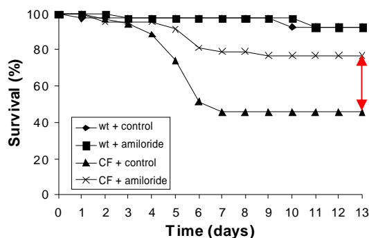
Figure 1: Early treatment with amiloride immediately after birth significantly reduces mortality in CF-transgenic mice (red arrow)
