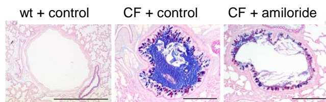
Figure 2: The congestion of the lung with mucus in CF-transgenic mice can be effectively treated by an early amiloride therapy commencing in the first few days after birth up to 14 days after birth. AB-PAS staining. Scale bar = 500 \mu m (wt), und 200 \mu m (CF).
